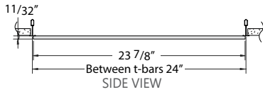
Flat felt shape, below t-bar shown.
