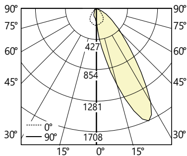
PHOTOMETRIC CURVE
