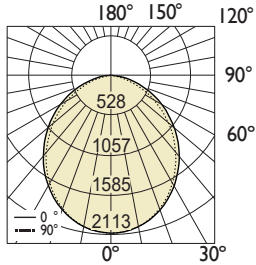
PHOTOMETRIC CURVE
