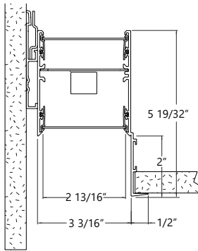
2RG 2" regressed DF Drywall flange
