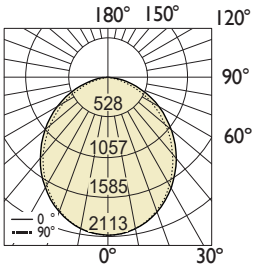
PHOTOMETRIC CURVE
