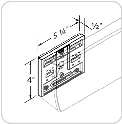
WB Wall Bracket Power side shown.
