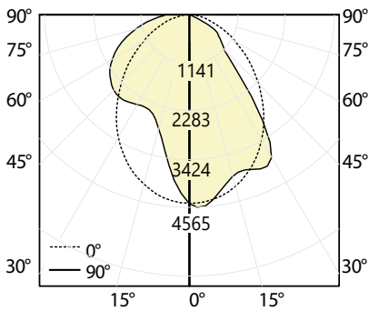
PHOTOMETRIC CURVE
