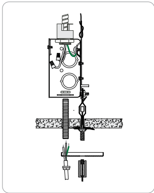
Power feed
