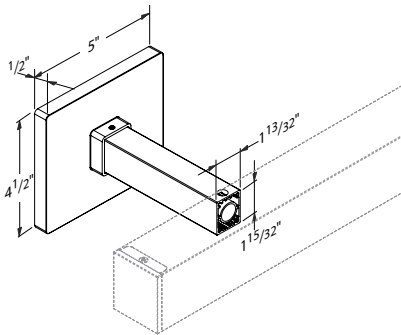
AM Arm mount shown.
