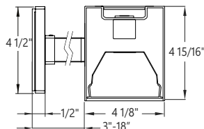
AM Arm mount shown
