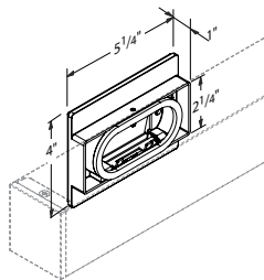
WB Wall Bracket Power side shown.
