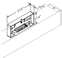
WB Wall Bracket Non-Power side shown
