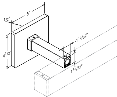
AM Arm mount shown.
