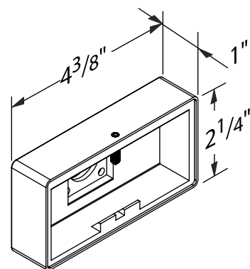
ISOMETRIC VIEW
