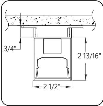
SB, BP Surface bracket with bird protection
