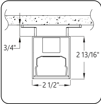
SB Surface bracket
