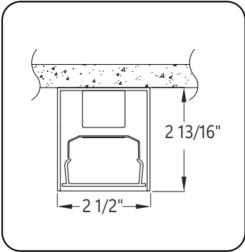
S Surface ceiling
