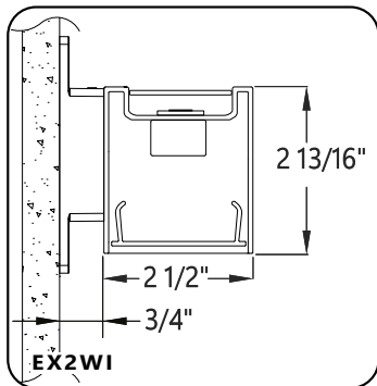
CL Clear lens ASO Asymmetric lens
