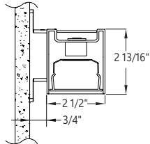
WB Wall bracket shown
