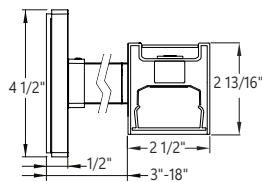
AM Arm mount shown
