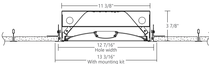
SECTION VIEW
